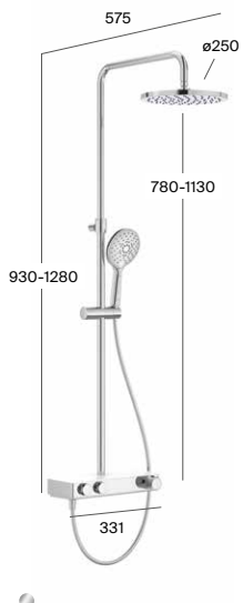
Shower column, 2 functions
