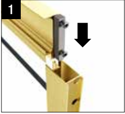
Align the horizontal and vertical profiles together.
