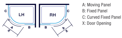
1 Door Offset Quadrant
