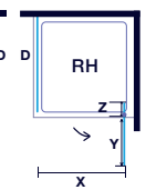
Pivot Door with Side Panel
