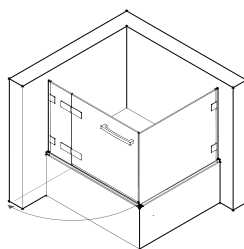
Wall Hinge Door with Inline Panel & side Panel
