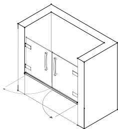
Wall Hinge Door in Recess
