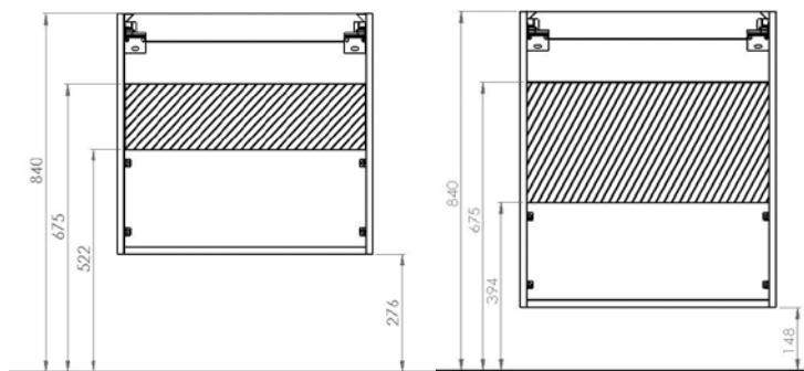
FITTED RANGE (in mm)
