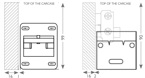
FIXING BRACKET DETAIL (in mm)
