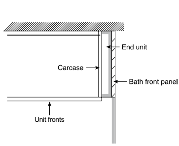
OVERHEAD VIEW
