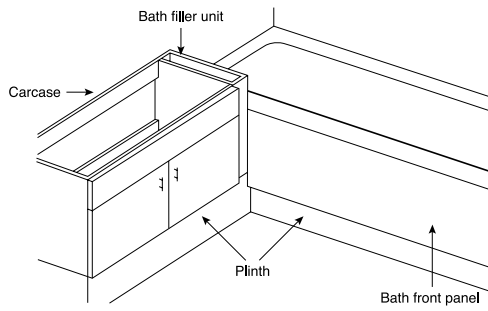
PERSPECTIVE
