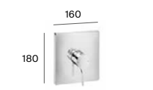
Built-in thermostatic mixer, 3-way diverter
