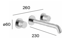
Twin-lever 3-taphole basin mixer, L-Size N
