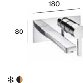
Built-in basin mixer
