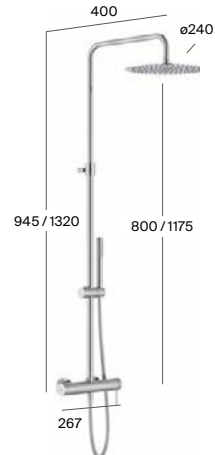
Shower column N
