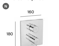
Built-in thermostatic bath-shower mixer, 2-way diverter. Roca Box Universal required
