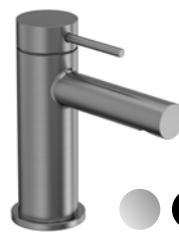
Anthem Mini Basin Mixer with Click Waste Minimum recommended pressure 0.2bar 42(w) x 143(h) x 136(d)mm
