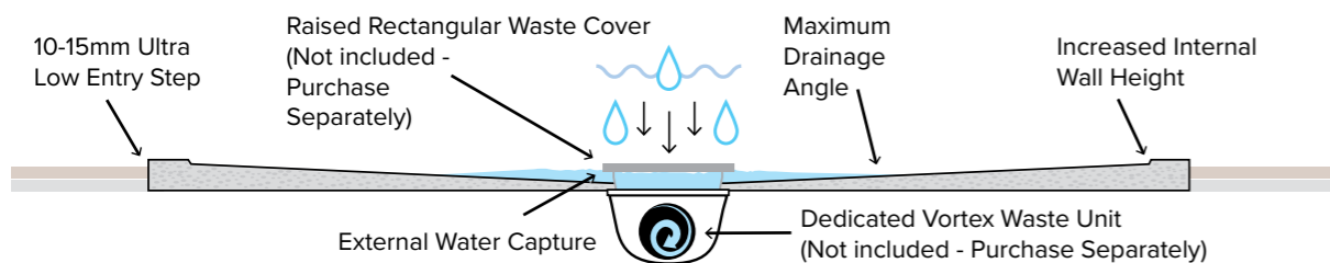
25mm High - Elementary Anti-Slip Stone Resin Shower Tray & Waste (Purchase Separately)
