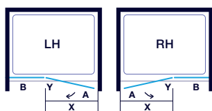
Hinge and Inline Door a Recess
