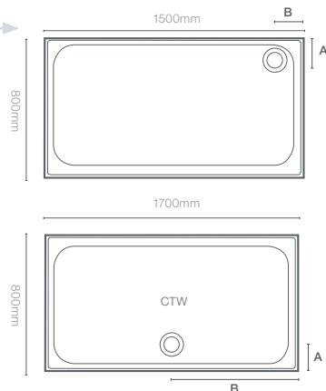
Waste is centred for 1700 x 800, 1700 x 900 and 1800 x 800 trays
