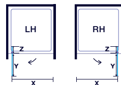
Pivot Door in Recess
