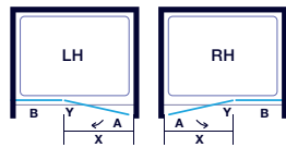
Hinge and Inline Door in Recess
