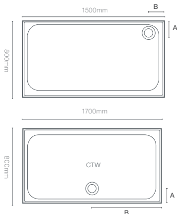
Waste is centred for 1700 x 800 / 1700 x 900 & 1800 x 800 trays
