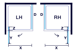
Pivot Door with Side Panel
